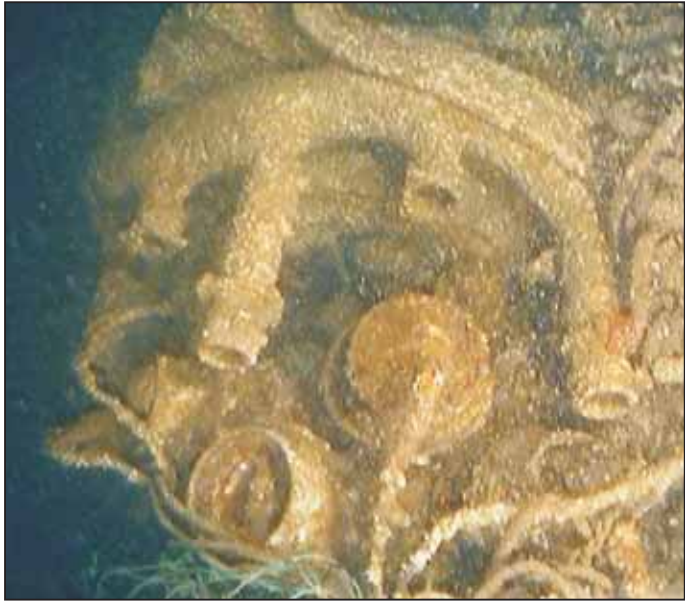
Plate C: Details of cylinders and exhaust collector ring on engine 2.
