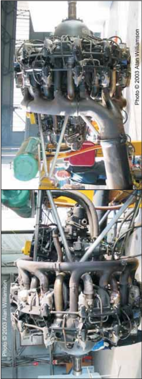
Plate A: Photographs of a Pratt & Whitney R-1830 Twin Wasp engine
