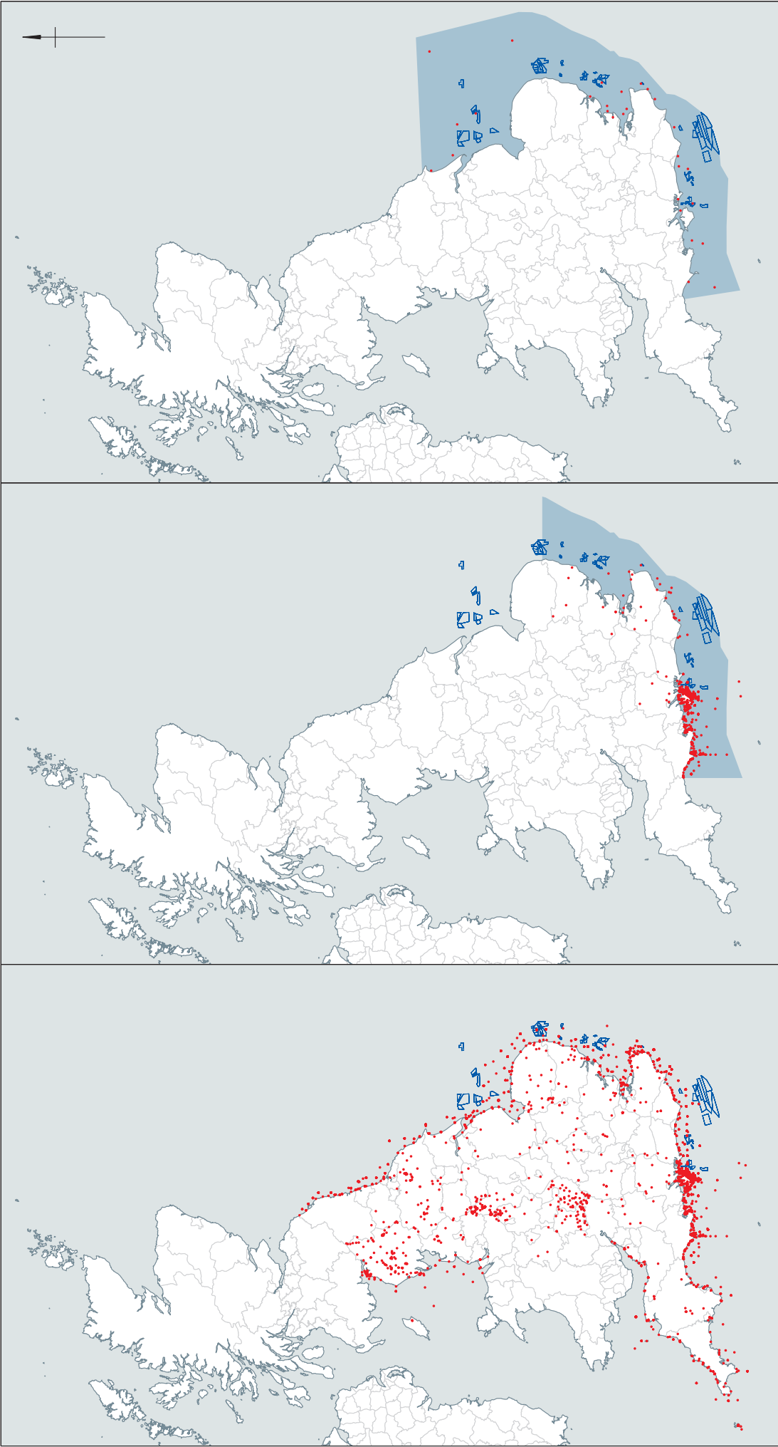
A: Known aircraft sites (NMR/SMR/HER data)
